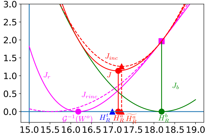
Figure 2.6: Example of output of the demo program.
