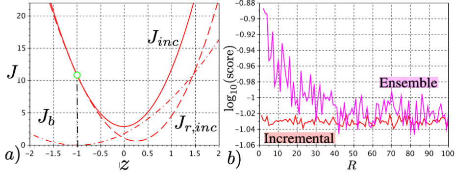
Figure 4.1: a) Plot of J_{inc} , J_b and J_{r,inc} as a function of z . b) Comparison of the scores of the incremental method and its ensemble approximation for the estimation of the true state.
