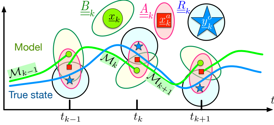
Figure 3.4: Extended Kalman filter.
