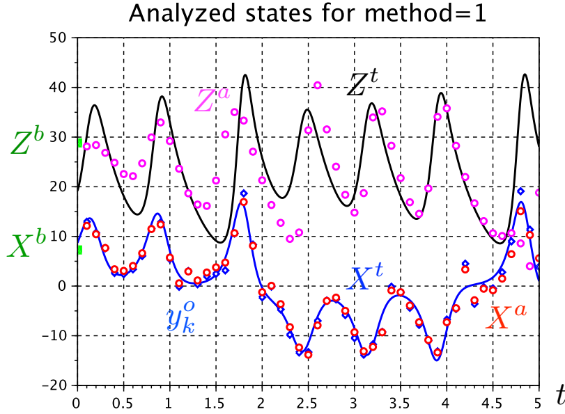
Figure 4.7: Chain of BLUE with a constant \underline{B} : analyzed states X_k^a (low red circles) and Z_k^a (high pink circles) for the observation times t_k for k = 1, \dots, 50 . The initial guess X^b and Z^b are displayed in green for t = 0 .
