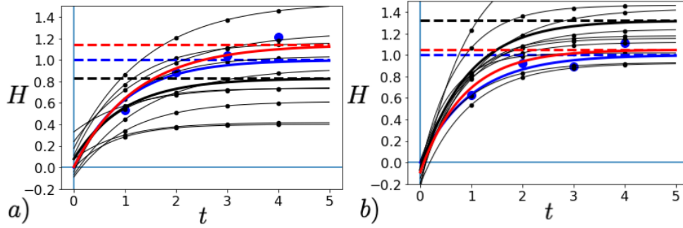
Figure 4.4: Two samples of the ensemble method for the estimation of \underline{x}^t . Blue: true state trajectory. Black: background trajectory and its ensemble perturbations. Red: trajectory of the analysis.
