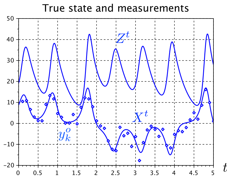
Figure 4.6: True state X^t(t) and Z^t(t) (solid lines) and measurements y^o(t_k) for i = 1, \dots, 50 (diamonds).
