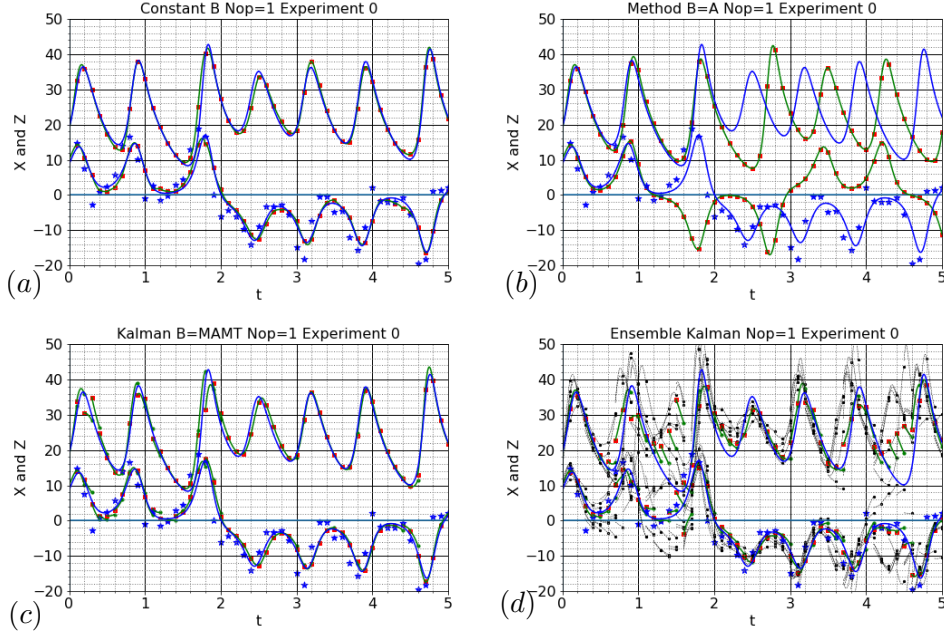
Figure 4.8: Comparison of four methods on a single experiment. a) 3D-Var with fixed \underline{B} . b) 3D-Var with \underline{B} replaced by \underline{A} . c) Kalman filter. d) Ensemble Kalman filter.
