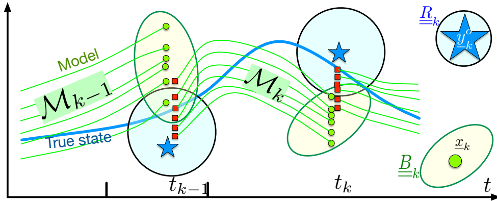
Figure 3.5: Ensemble Kalman filters.
