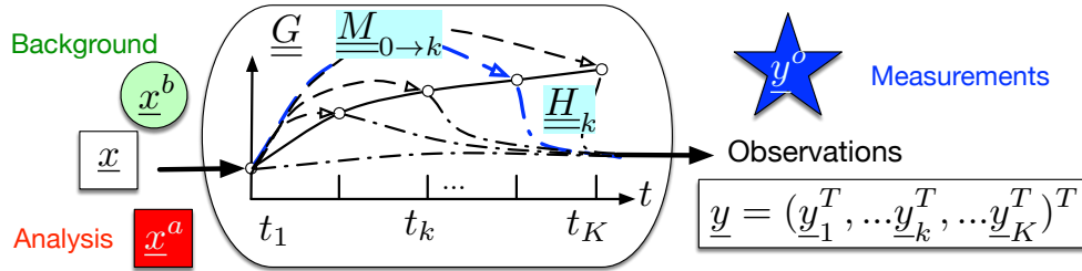
Figure 3.2: Linear 4D-Var data assimilation method.
