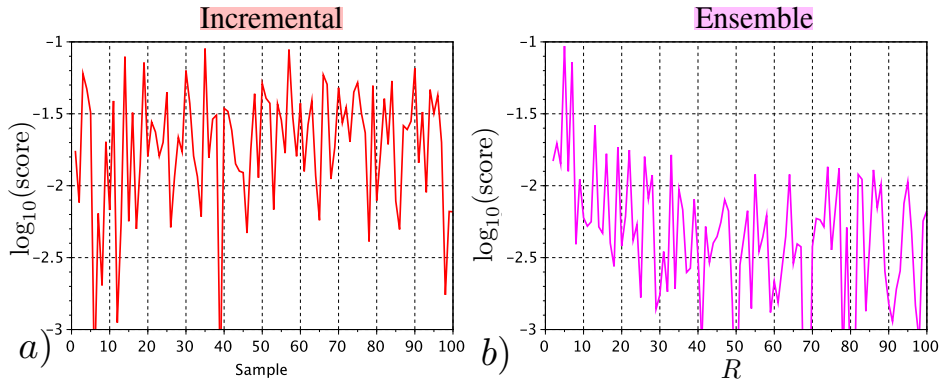
Figure 4.3: Scores of a) the incremental method and b) its ensemble approximation for the estimation of the true state.
