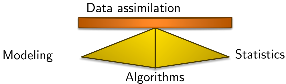
Figure 1: Data assimilation is at the crossroad of several topics.
